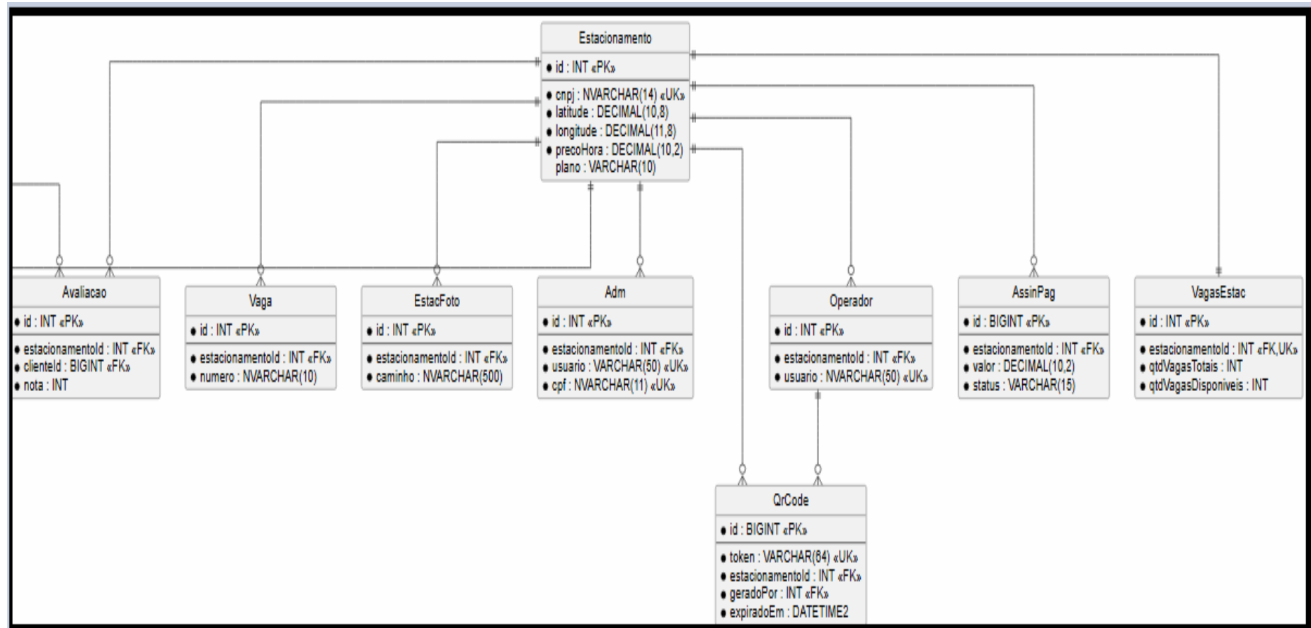
Figura 27 - Diagrama DER (2/2)
